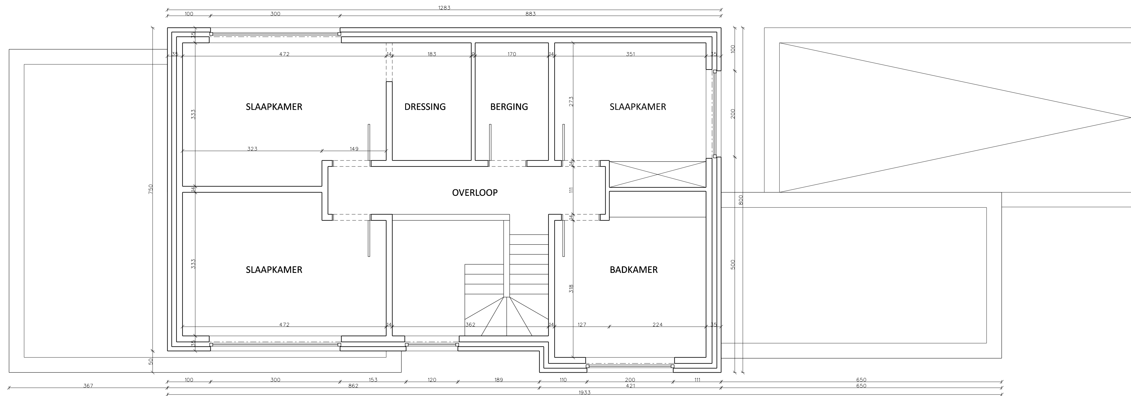
PLAN VERDIEPING 0 1m 2m 3m 4m 5m
